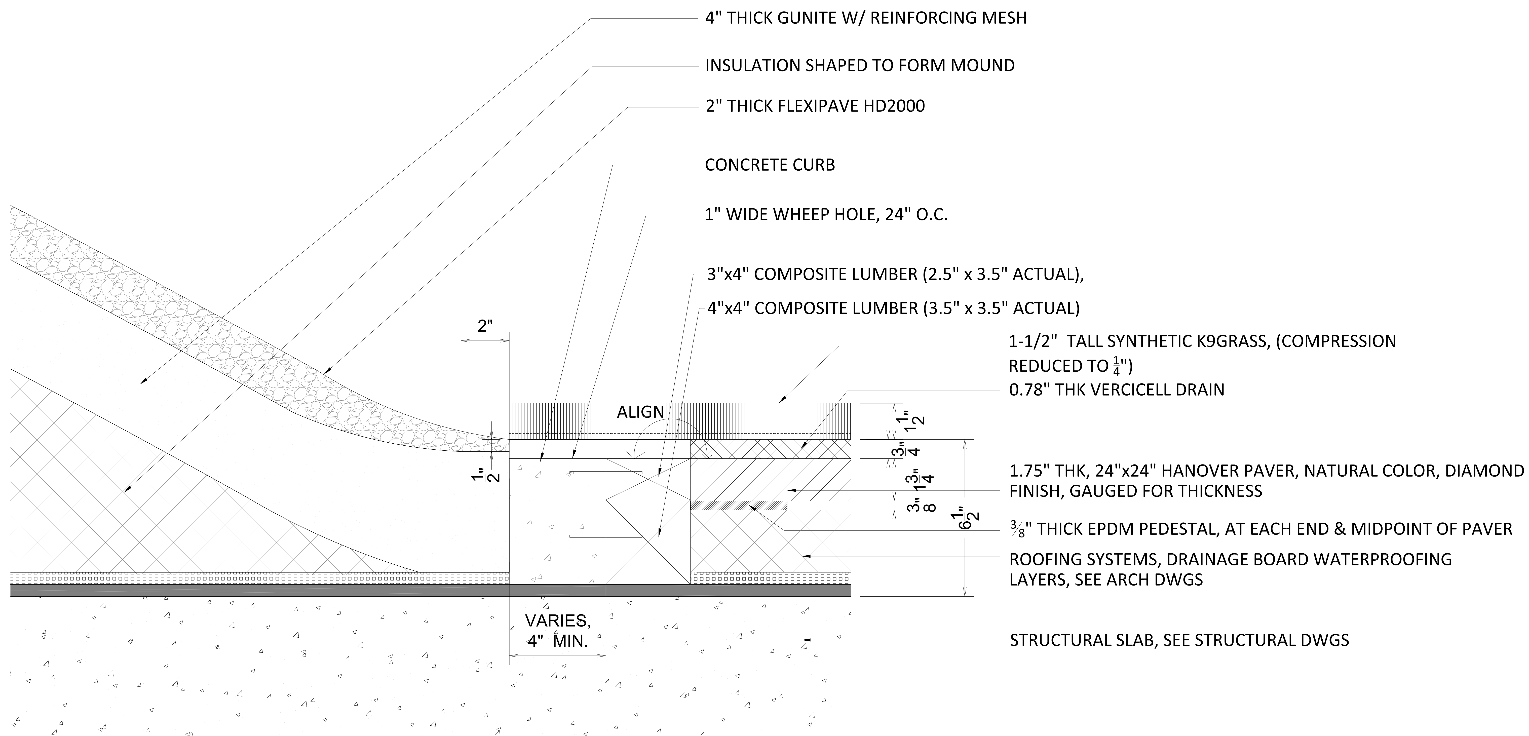
B MOUND DETAIL- WEEP HOLE AT TOP SCALE: 1-1/2" = 1'-0"
