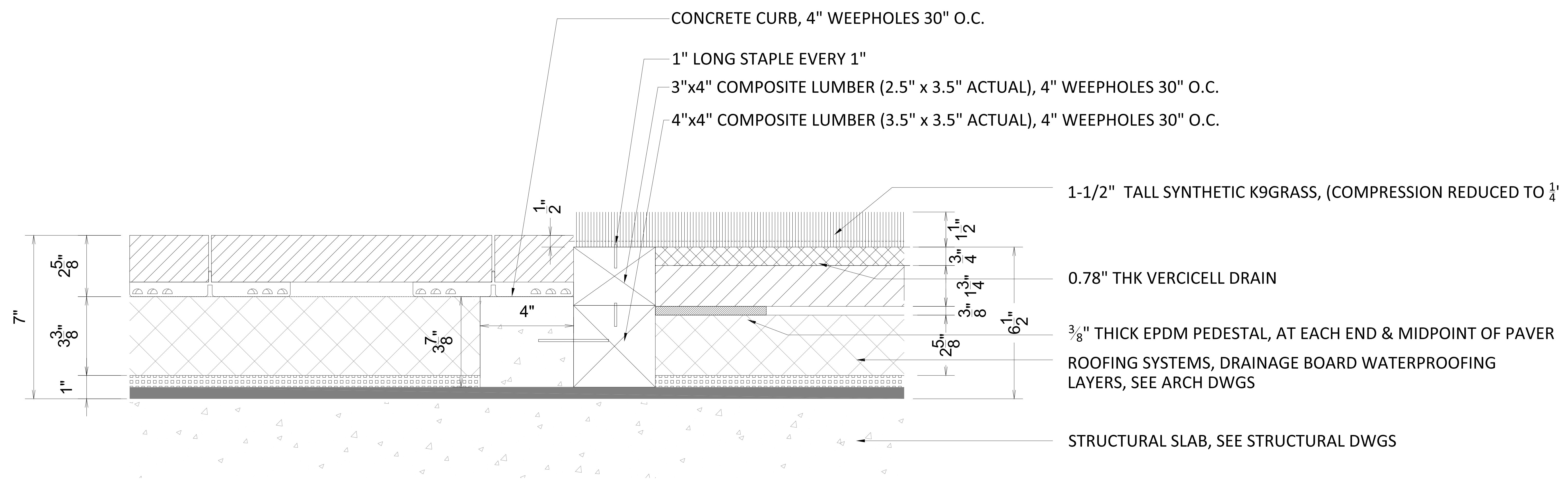
A TURF TO PAVER TRANSITION SCALE: 1-1/2" = 1'-0"
