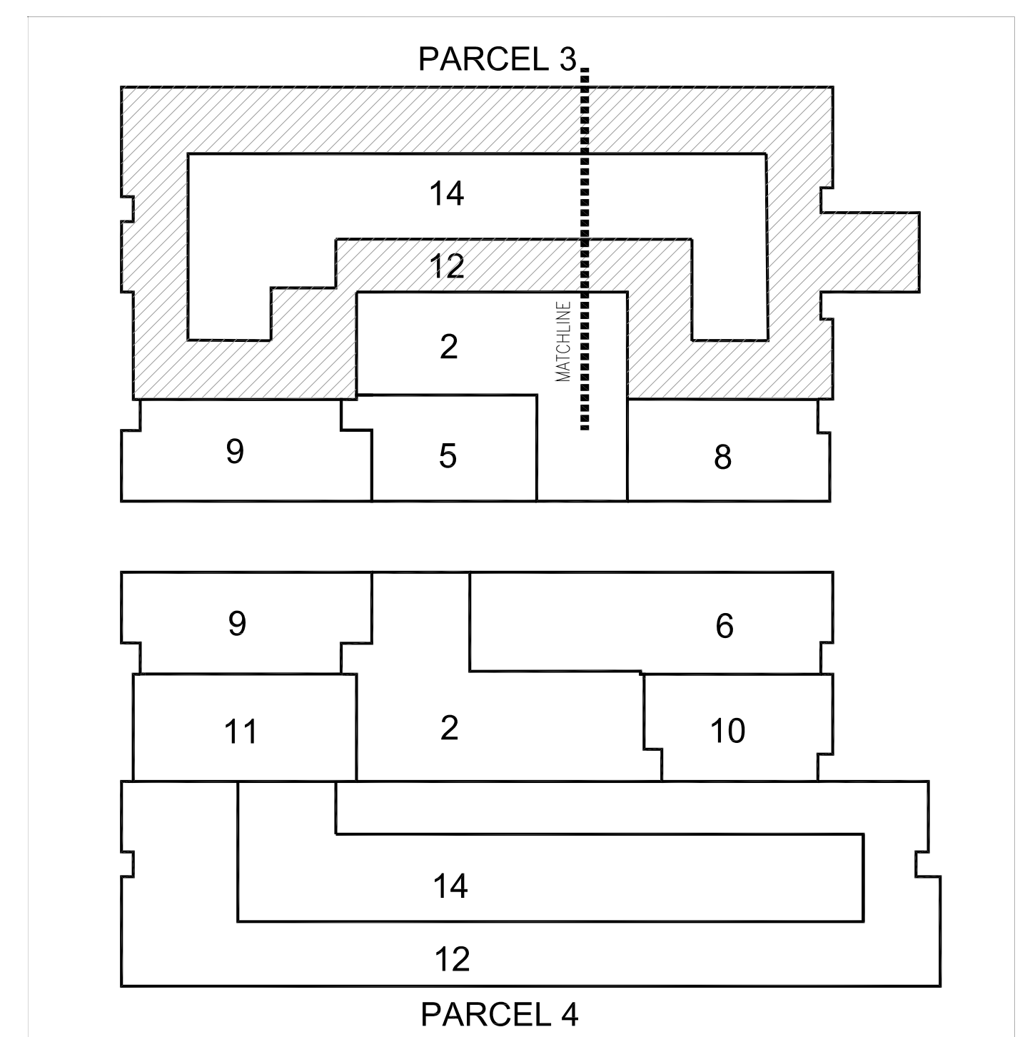
LEVEL 12 ROOF TERRACE (PARCEL 3) - SITE + MATERIAL PLAN SCALE: 1/4" = 1'-0"
