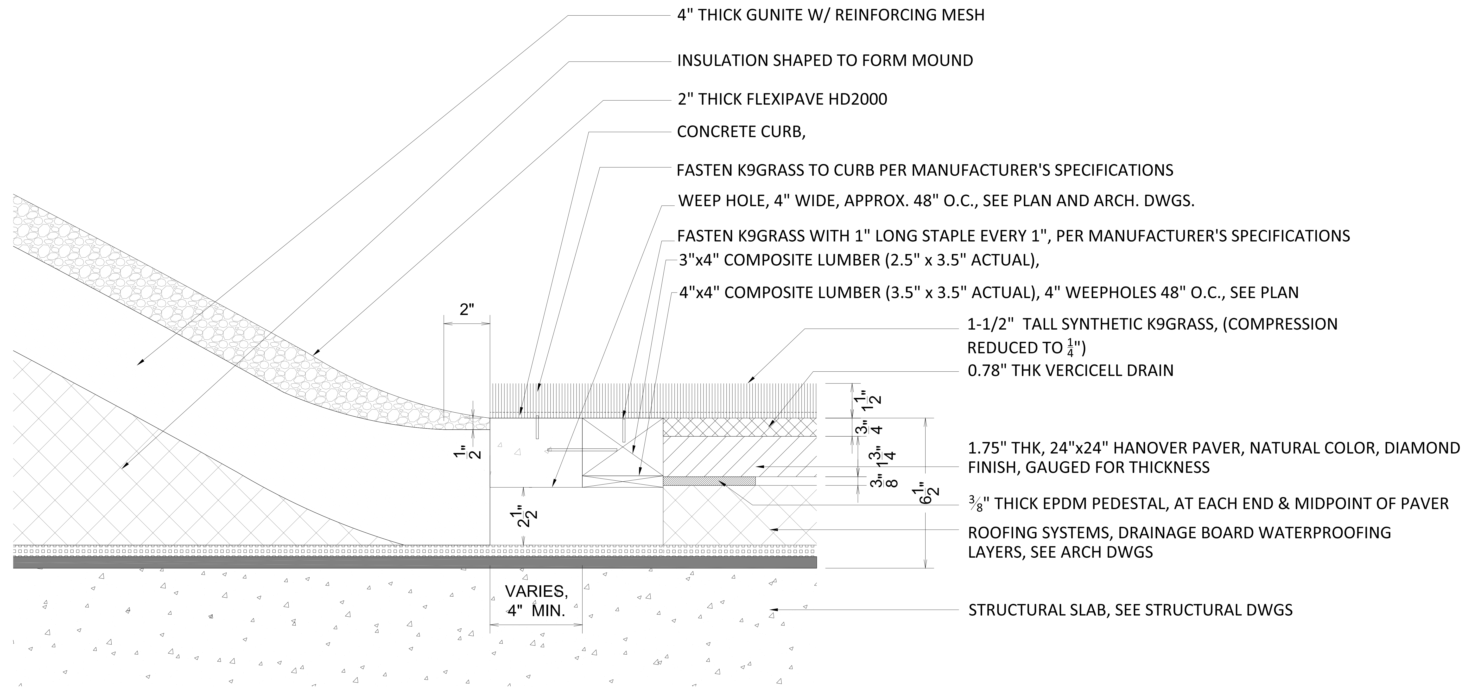
B MOUND DETAIL- WEEP HOLE AT BOTTOM SCALE: 1-1/2" = 1'-0"
