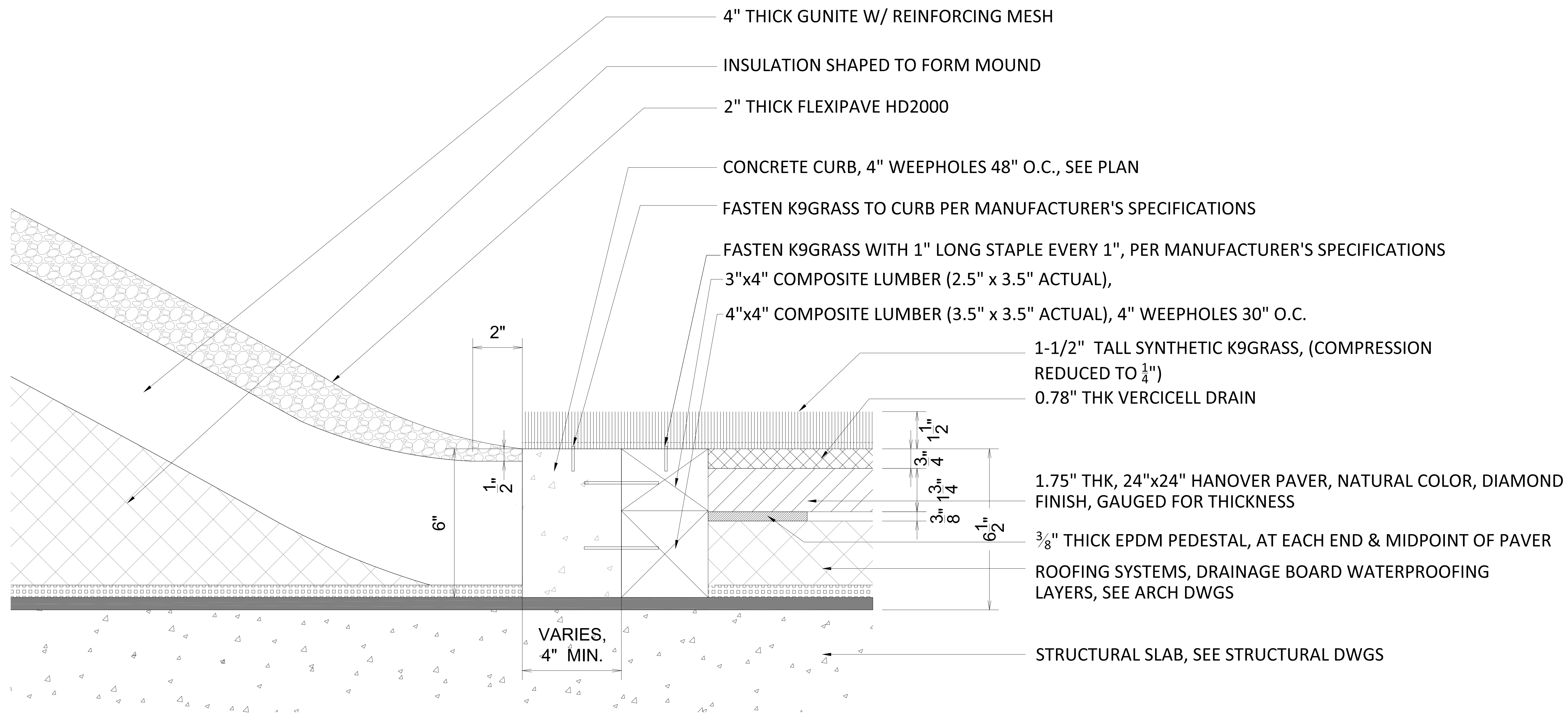
A MOUND DETAIL- NO WEEP HOLE SCALE: 1-1/2" = 1'-0"
