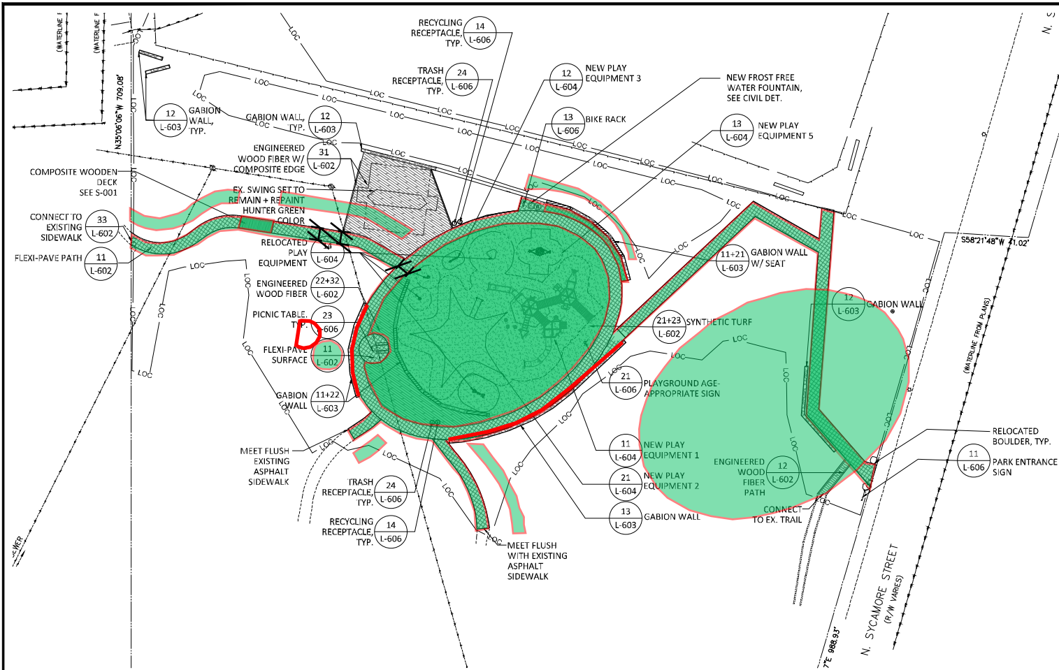
1 SITE + MATERIAL PLAN 1"=20'-0"
